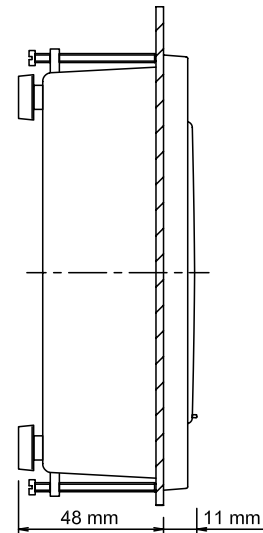
Panel-mounted MULTICAL® 6M2 seen from the side
