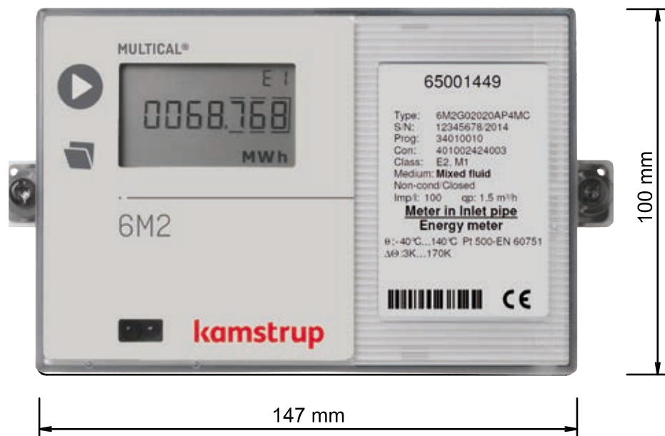
Front dimensions of MULTICAL® 6M2
