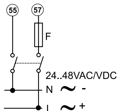
Fig. 23 L option. F = 250 \text{ V}, 200 \text{ mA}
