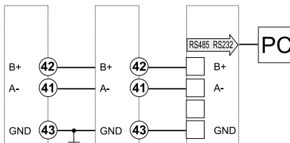
Fig. 28 Port RS485
