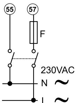
Fig. 21 D option. F = 250 \text{ V}, 50 \text{ mA}
