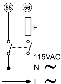
Fig. 22 D option. F = 250 \text{ V}, 100 \text{ mA}
